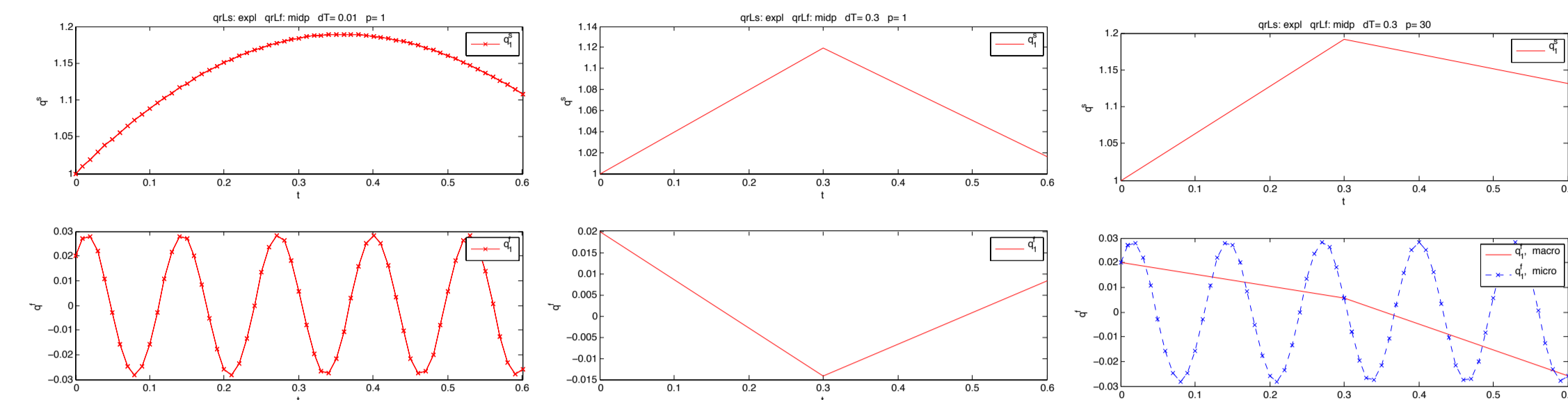
Configuration of first slow and first fast variable. Left: Reference solution computed with variational integrator and time step \Delta T = 0.01 . Middle: Variational integrator with time step \Delta T = 0.3 . Right: Variational multirate integrator with macro time step \Delta T = 0.3 and micro time step \Delta t = 0.01 .
