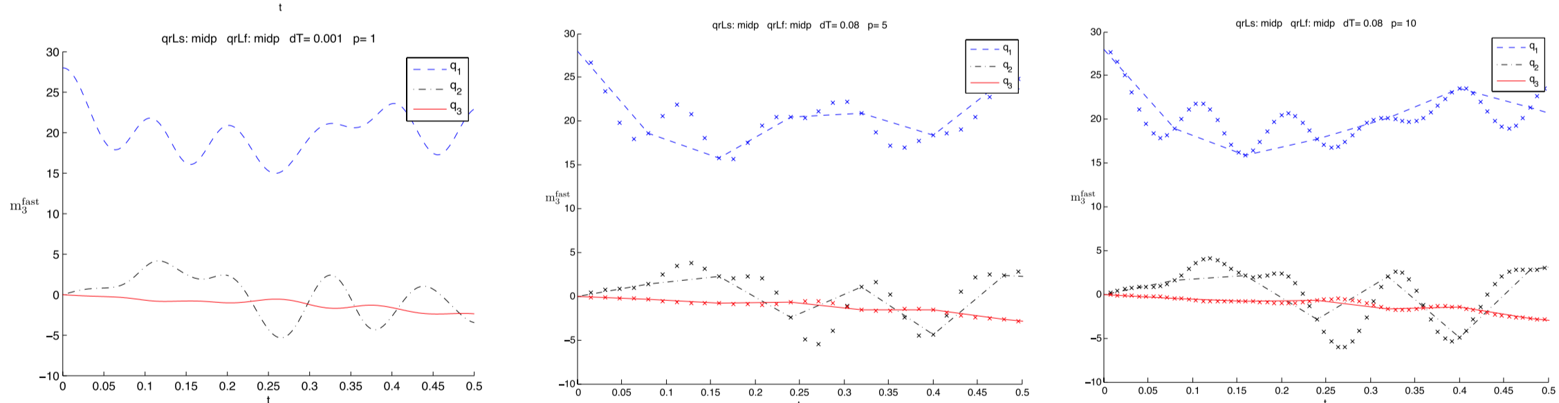
Configuration of second fast variable. Left: Reference solution computed with variational integrator and time step \Delta T = 0.001 . Middle: Variational multirate integrator with macro time step \Delta T = 0.08 and p = 5 . Right: Variational multirate integrator with macro time step \Delta T = 0.08 and p = 10 .
