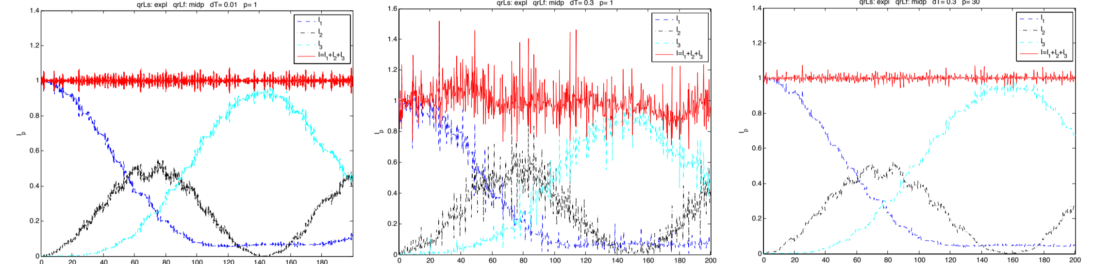
Energy in stiff springs (adiabatic invariant) Left: Reference solution computed with variational integrator and time step \Delta T = 0.01 . Middle: Variational integrator with time step \Delta T = 0.3 . Right: Variational multirate integrator with macro time step \Delta T = 0.3 and micro time step \Delta t = 0.01 .
